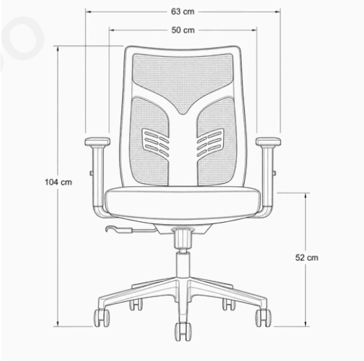
VISTA FRONTAL
